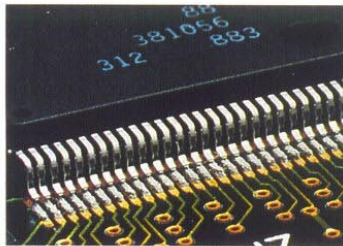
The LSM makes it possible to verify the quality of solder paste printing on critical fine-pitch sites.
